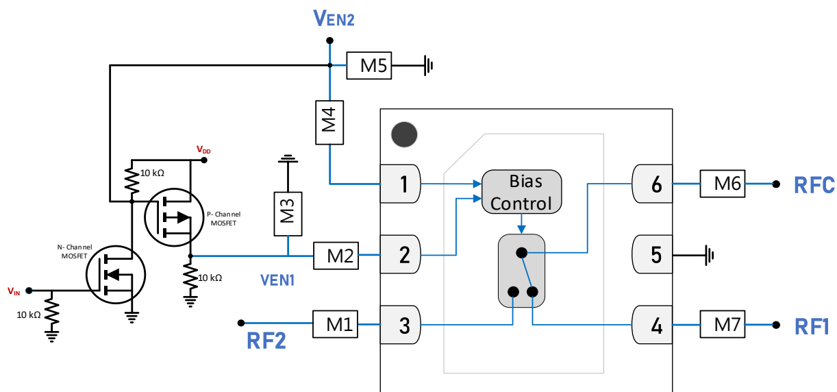
GRF6004 Standard Evaluation Board Schematic
