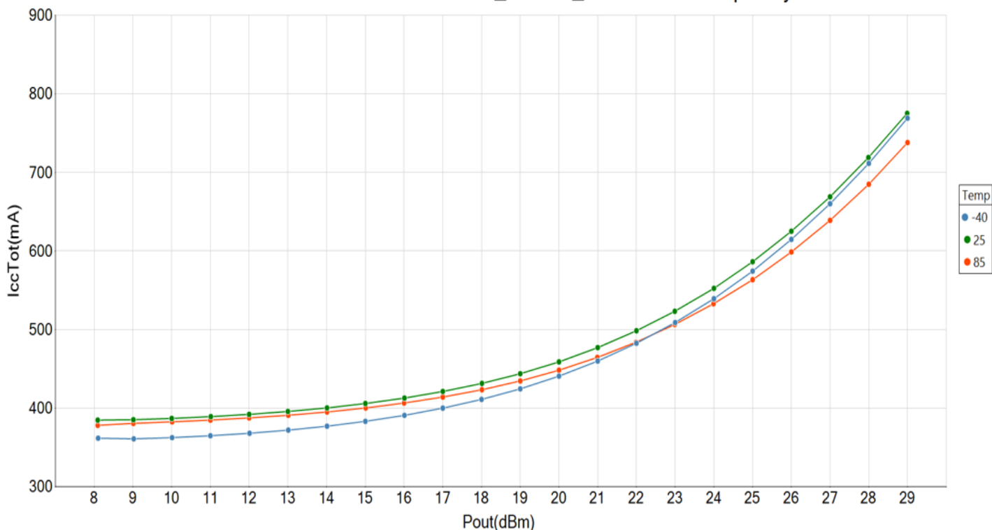
GRF5618 IccTot vs Pout at Modulation = LTE_20MHz_100RB and Frequency = 1880 MHz
