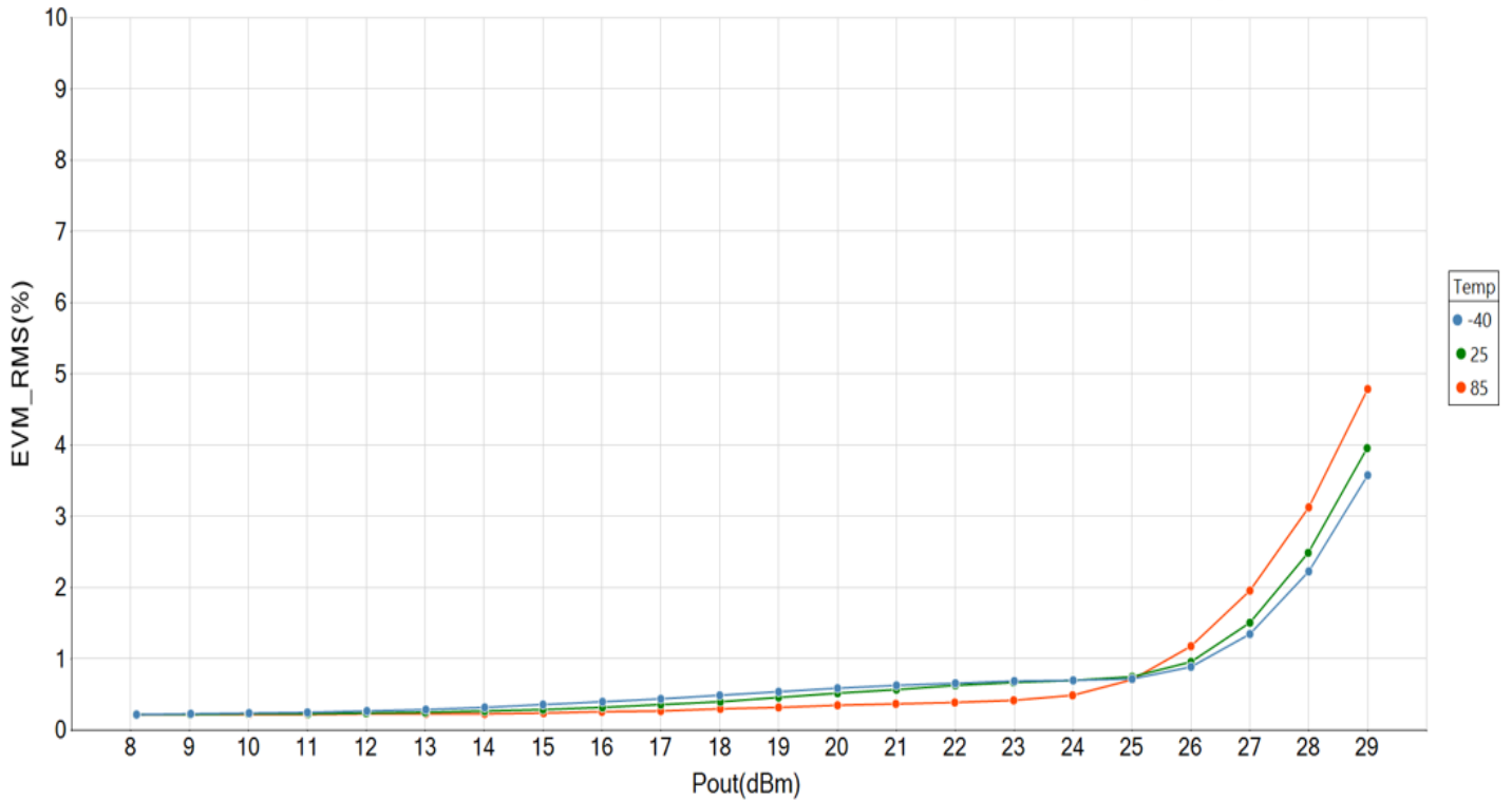
GRF5618 EVM_RMS vs Pout at Modulation = LTE_20MHz_100RB and Frequency = 1880 MHz
