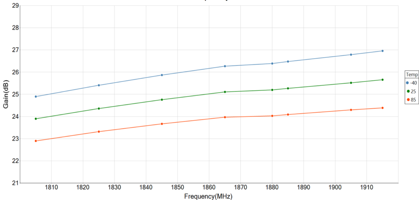
GRF5618 Gain vs Frequency at Pin = -25 dBm
