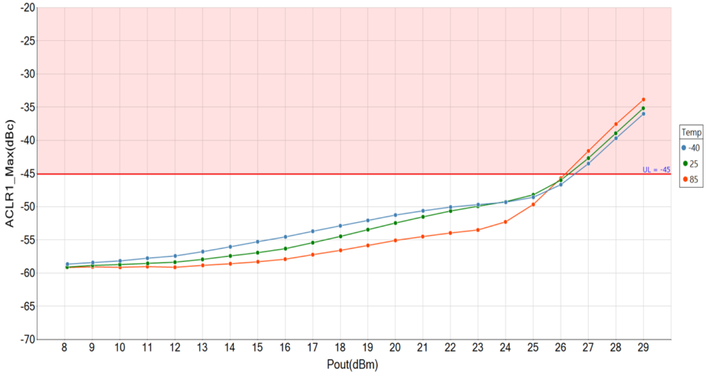
GRF5618 ACLR1 vs Pout at Modulation = LTE_20MHz_100RB and Frequency = 1880 MHz
