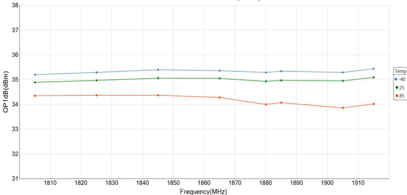
GRF5618 OP1dB vs Frequency
