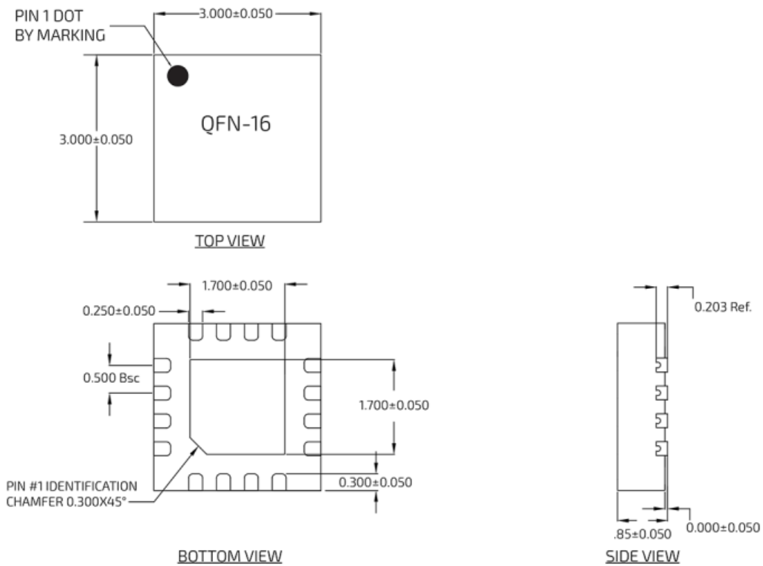
3 x 3 mm QFN-16 Package Dimensions
