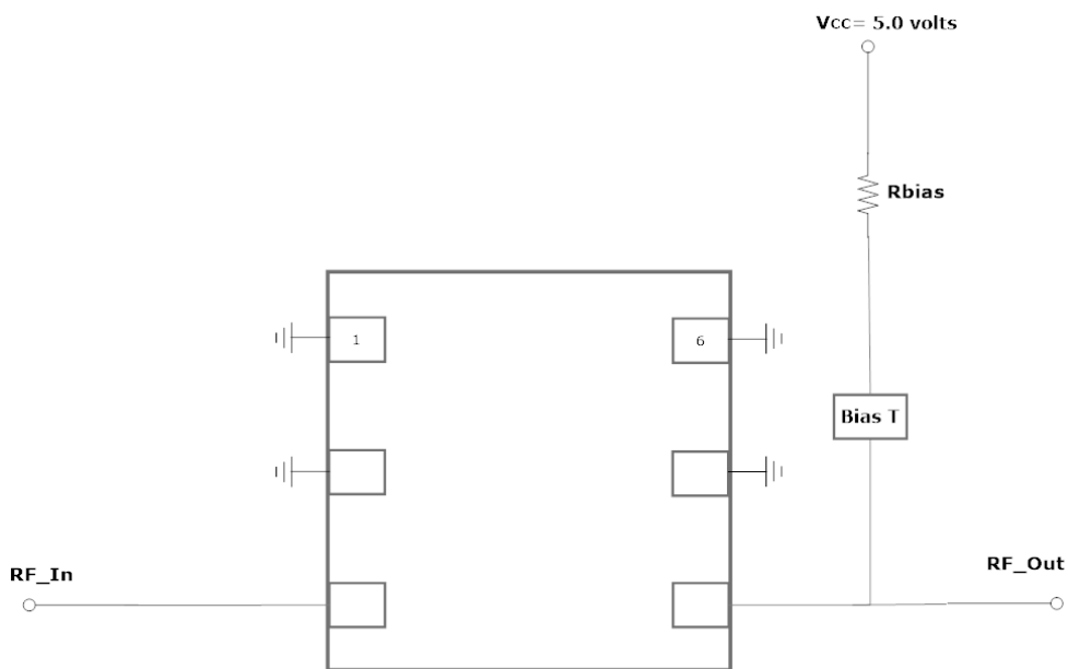
GRF3014 Standard 5-Volt Test Schematic
