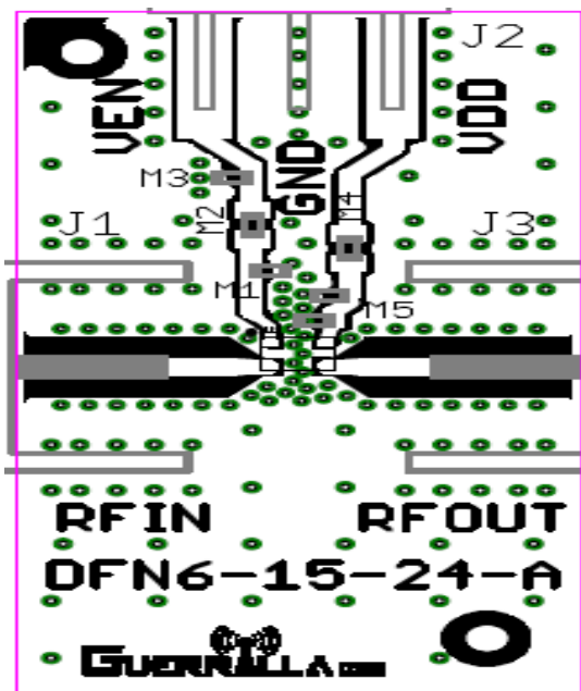
GRF3014 Evaluation Board Assembly Diagram
