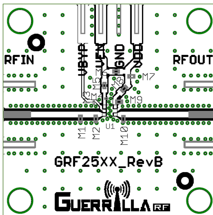
GRF2501W Evaluation Board Assembly Diagram
