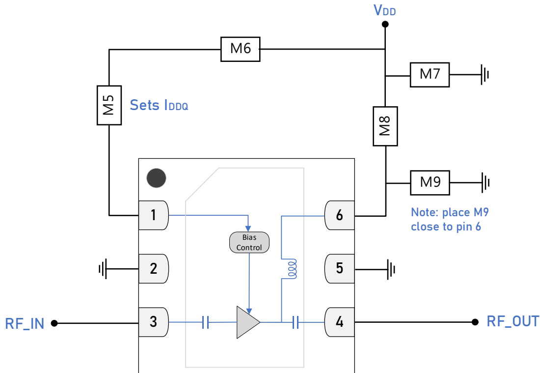
GRF2501W Standard Evaluation Board Schematic
