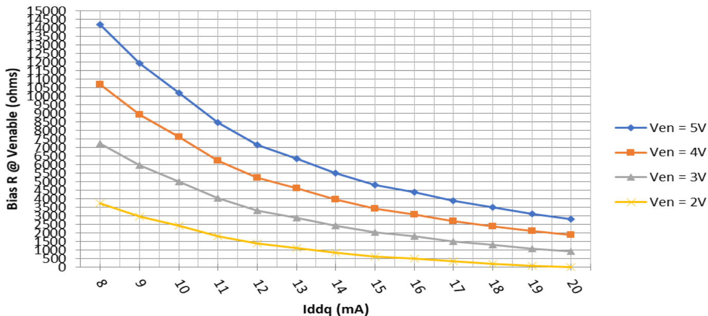
GRF2243 w/Vdd = 5.0V: Required Bias R @ Venable vs. Iddq
