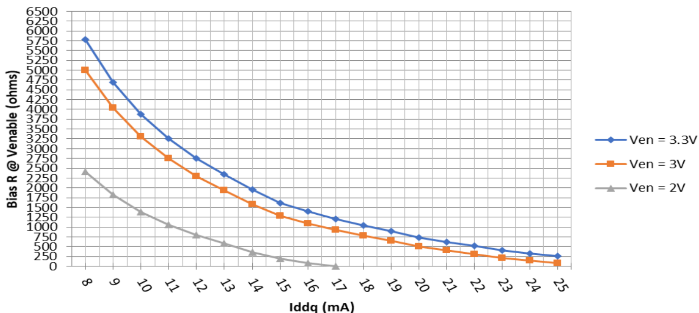
GRF2243 w/Vdd = 3.3V: Required Bias R @ Venable vs. Iddq
