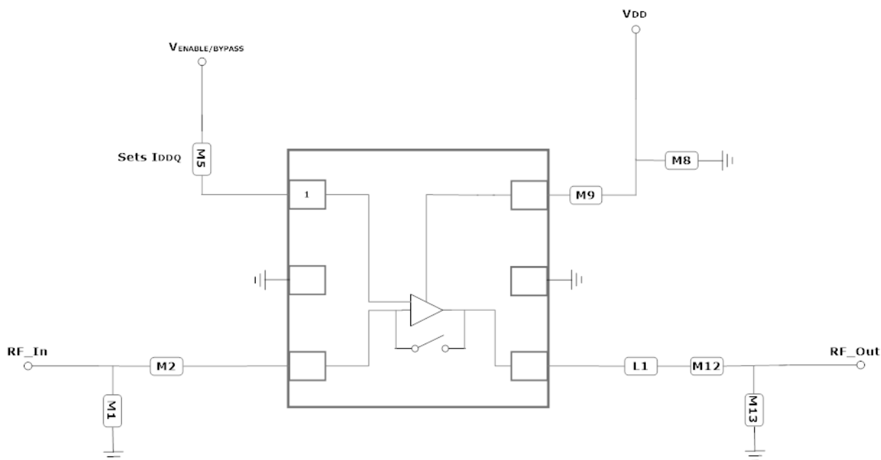
GRF2243W Application Schematic
