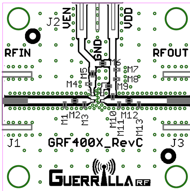
GRF2243W Evaluation Board Assembly Diagram
