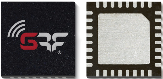
5.0x5.0 QFN-32
