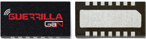
6.0x3.0 DFN-14
